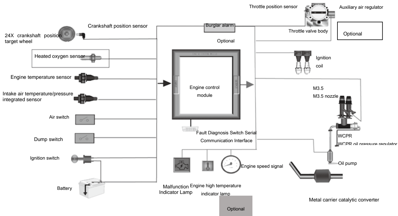
Structural schematic diagram of EFI system
