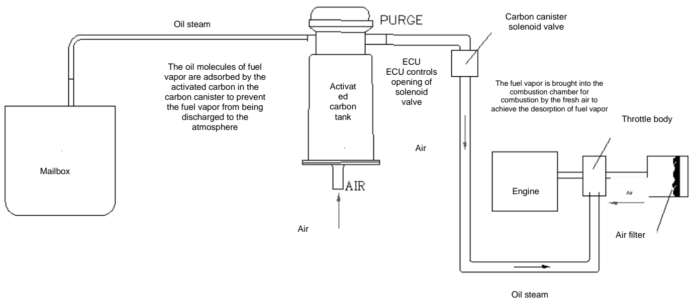
National emission and fuel evaporation working diagram
