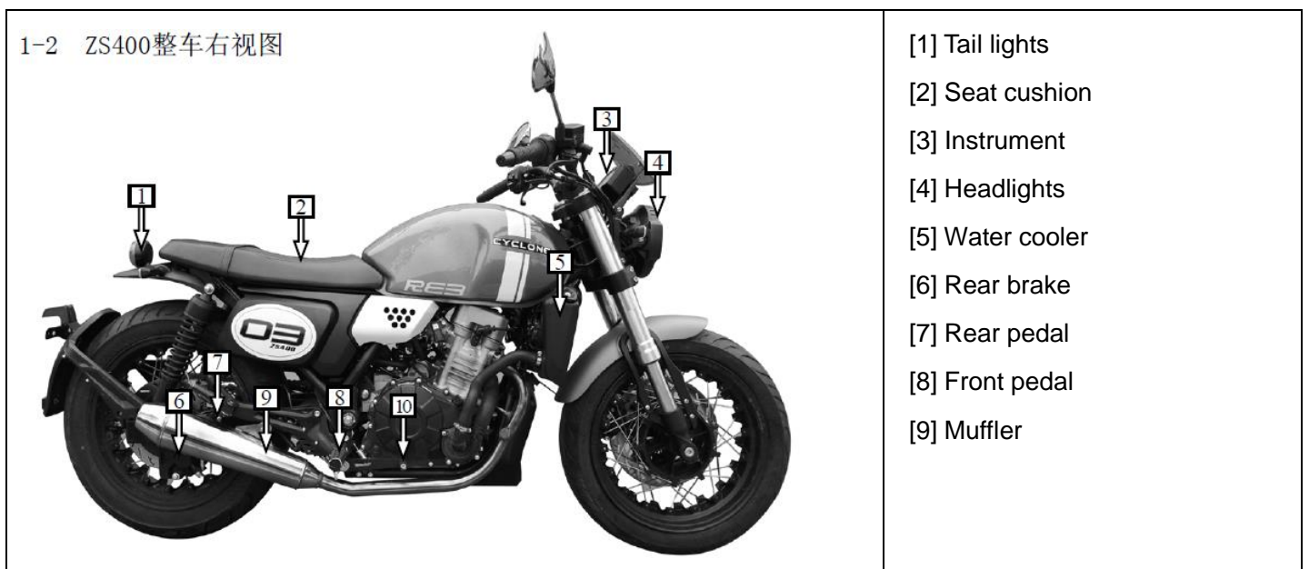
Fig. 1-2 Right side view of ZS400 complete vehicle
